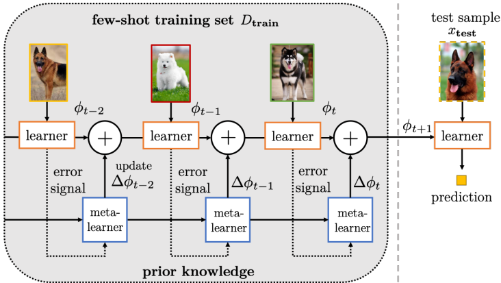
Fig. 15. Solving the FSL problem by learning the optimizer.
