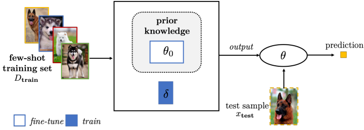
Fig. 13. Solving the FSL problem by fine-tuning existing parameter \theta_0 with new parameters.
