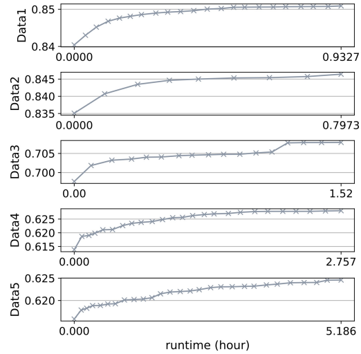
Figure 7: Validation AUC curves in real-business datasets.
